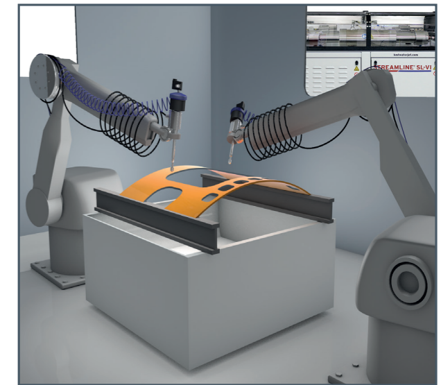
3D-Cutting Box with high pressure pump STREAMLINE SL-VI 100
